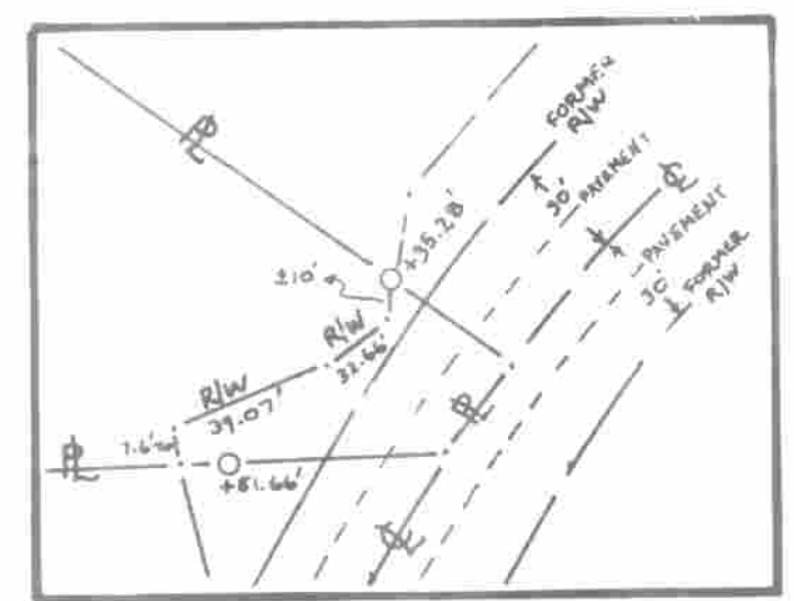
BLOW-UP OF 0.04 AC. OHIO STATE R/W (FROM STATE R/W PLANS: ATH-682- + 25-4-11, 16/17, 1/2)
