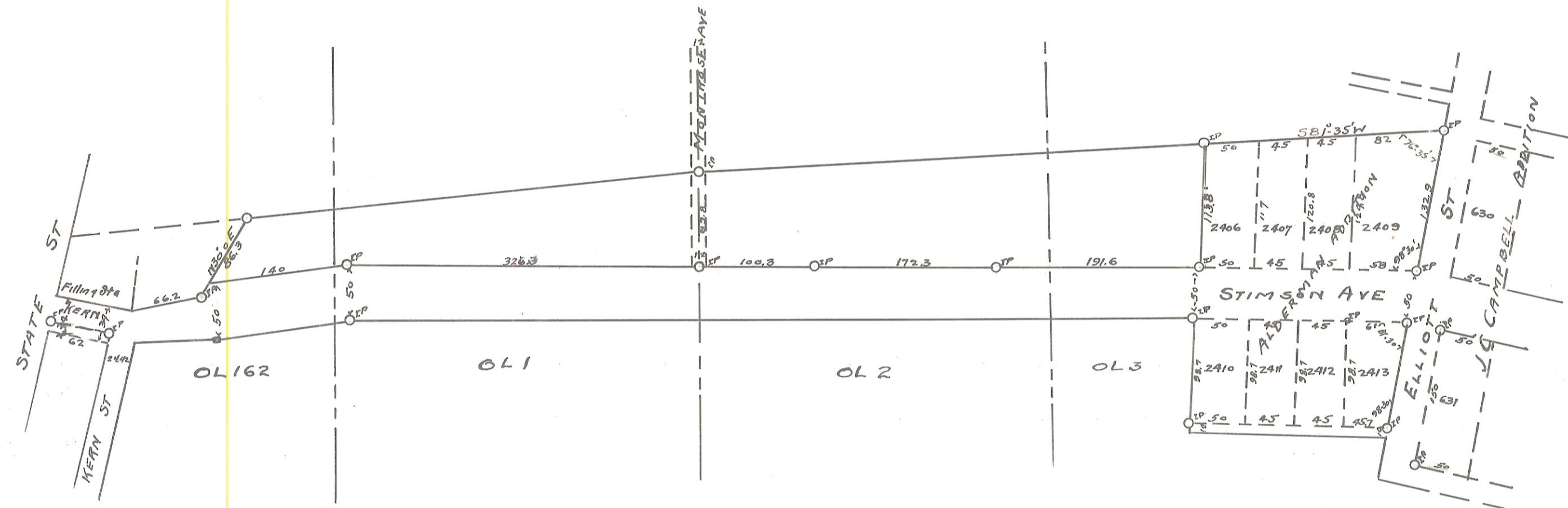
PROPOSED EXTENSION OF STIMSON AVE SCALE 1" = 100'
